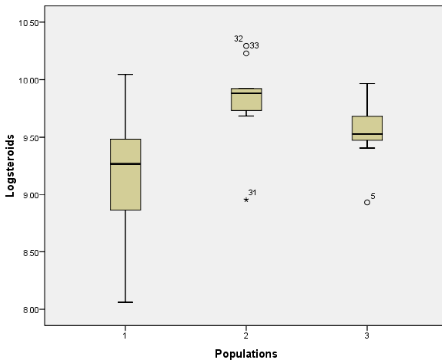
Fig 2. Boxplots of the five chemical groups (steroids, acids, alcohols, glycerolmonoethers, and monoglycerides) expressed as log abundance for the 3 populations, 1(Sinai), 2 (Siwa) and 3 (Abu Rawash). Populations 1 and 2 are different for all groups of chemicals, similarly 1 and 3 except for glycerolmonoethers.
