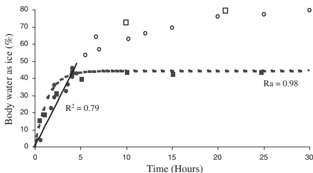
Fig. 1. The time course of ice accumulation in oviparous (circles) and viviparous (squares) lizards subjected to freezing at -3^{\circ}\text{C} . Open symbols correspond to the animals that died during freezing; data for these animals were not used in fitting the curves. A non-linear regression fitted the data from the viviparous strain. The hyperbolic plot: y=47.8(1-\exp^{-0.72x}) represent the best fit to the percentage of body water frozen in viviparous lizards over time. We give the "Ra" as the ratio between the totals of sums of squares explained by the regression and uncorrected (equivalent of the R^2 of a linear regression). The time course of ice accumulation from surviving oviparous individuals (those sampled between 0.5 and 5 hours of freezing exposure) followed a linear regression ( y=10.8x ; R^2=0.79 ; n=10 ).
